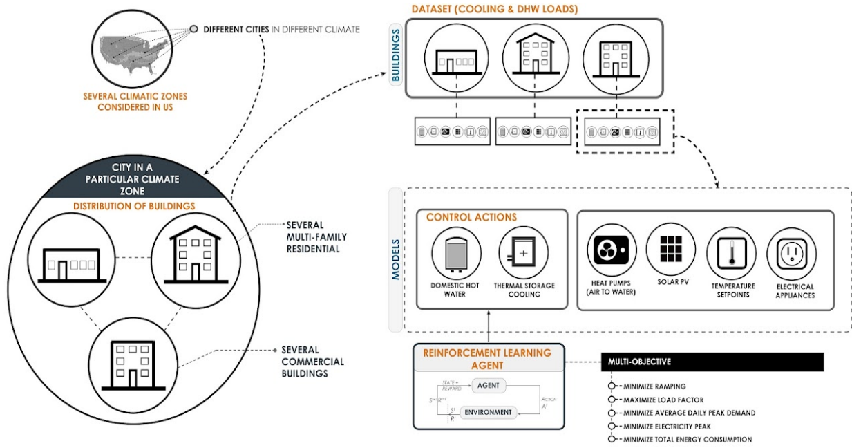
Fig. 2. CityLearn challenge architecture with multi-criteria optimization [16]
