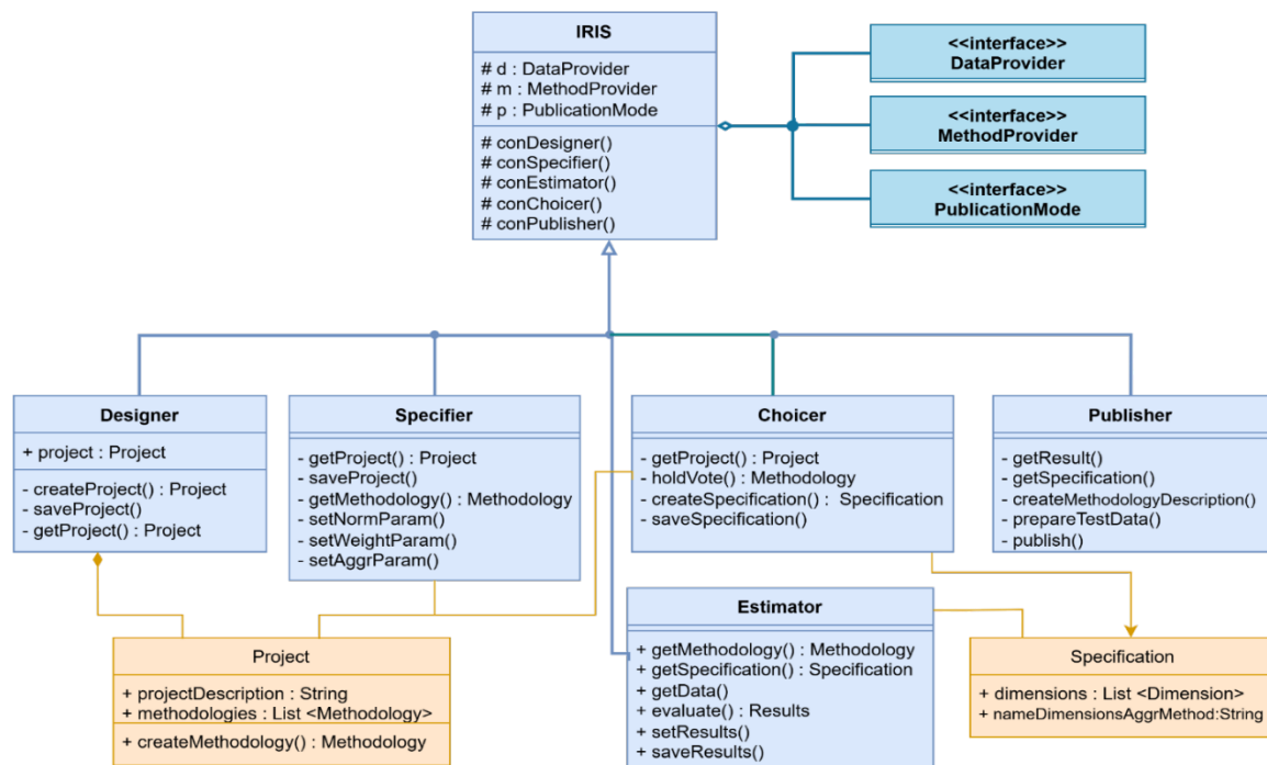
Fig. 2. Diagram of basic classes of the software system for evaluating the level of internationalization of a scientific institution
