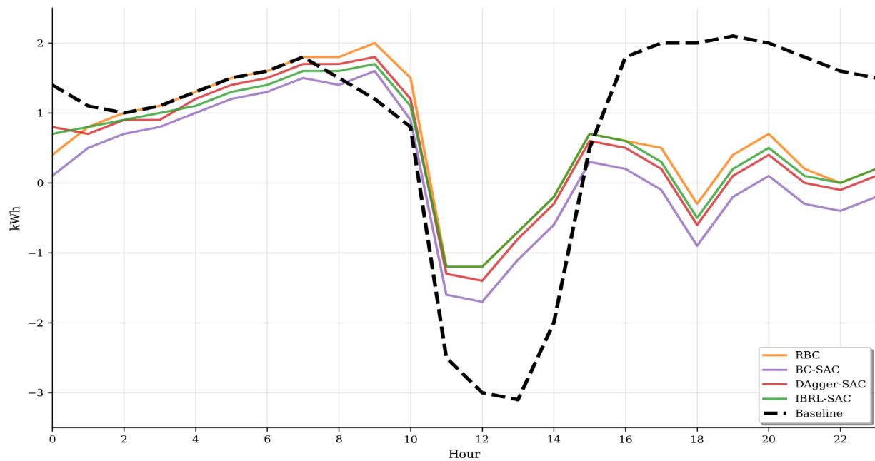
Fig. 6. Daily average load profiles for each IL algorithm
