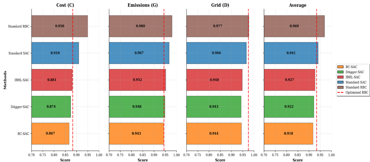
Fig. 5. Performance comparison across key CityLearn metrics
