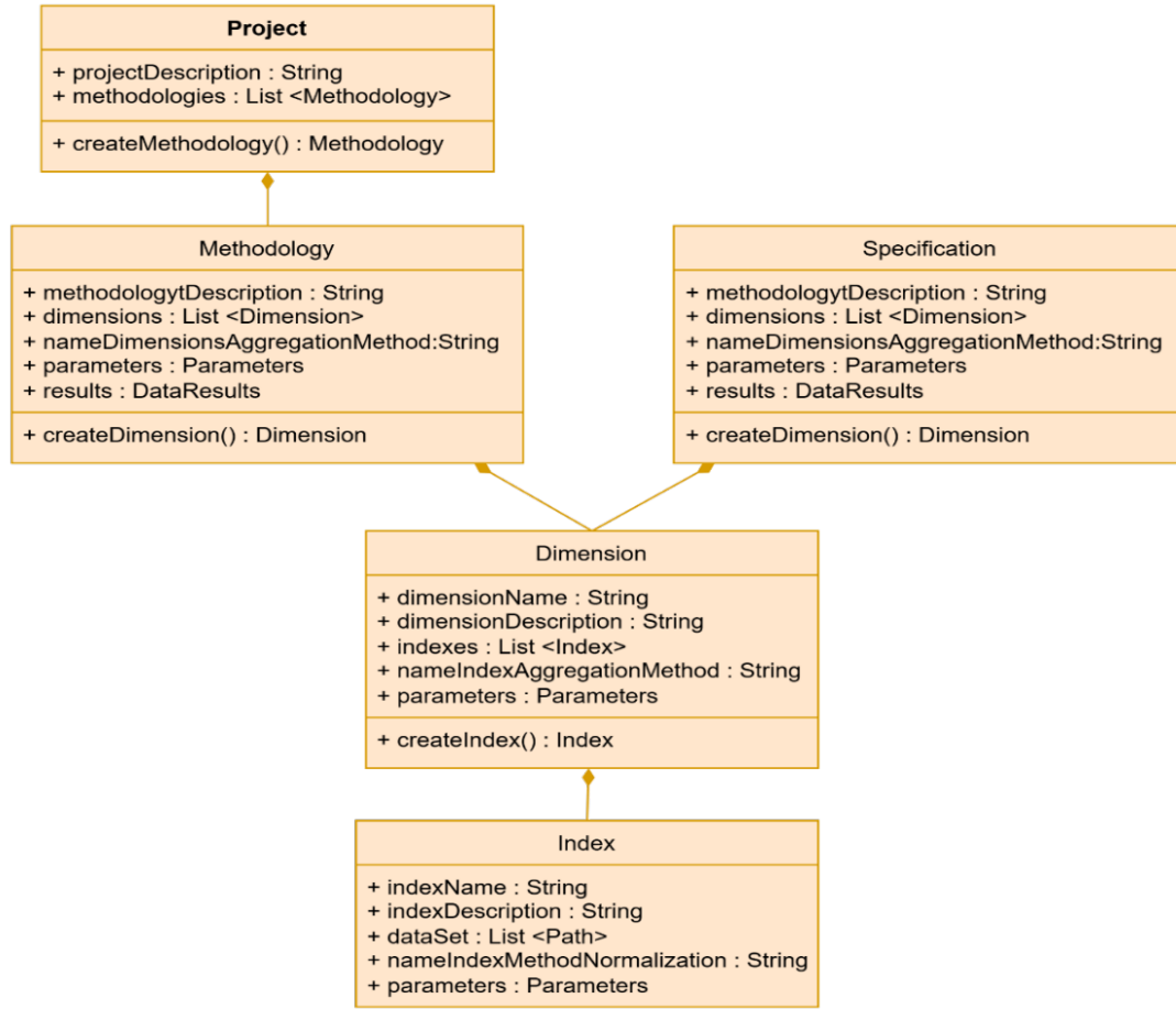
Fig. 3. Structure of the main artifact classes
