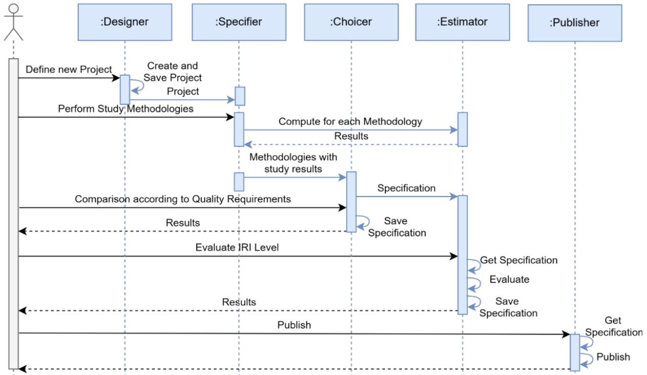
Fig. 4. Software system sequence diagram
