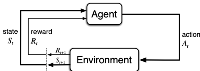
Fig. 1. Reinforcement learning agent-environment interaction schema [14]
