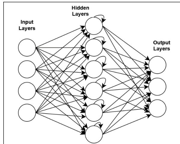
Fig. 1. RNN scheme
