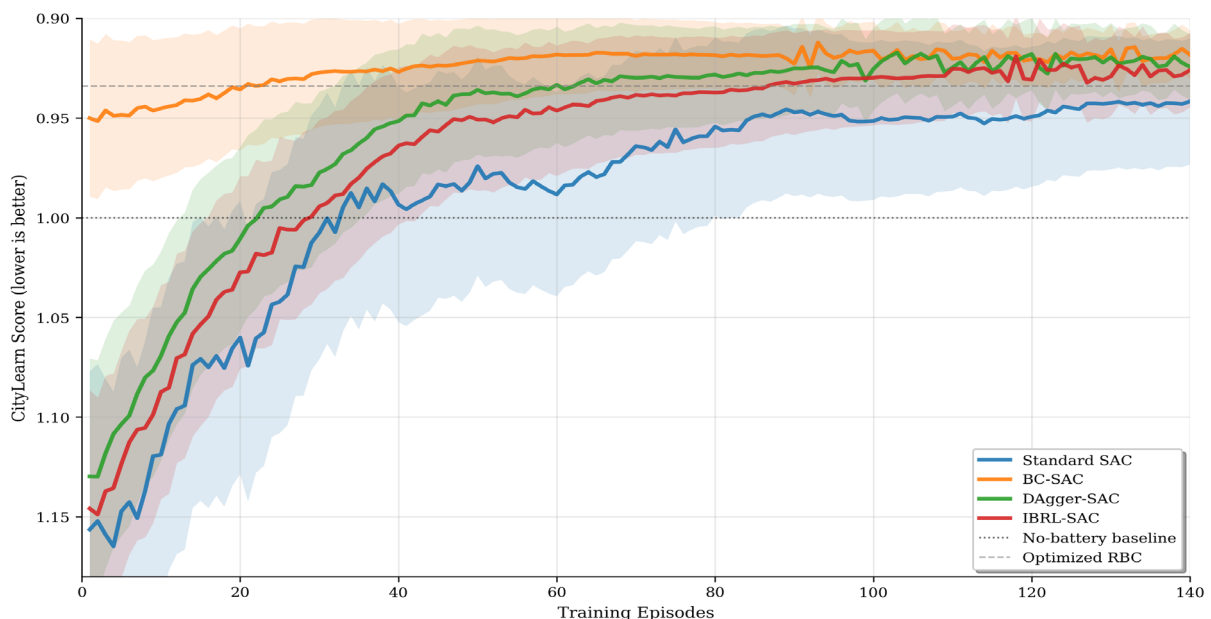
Fig. 4. Convergence speed comparison across imitation learning methods
